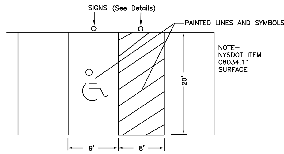
TYPICAL ADA PARKING DETAIL NOT TO SCALE
