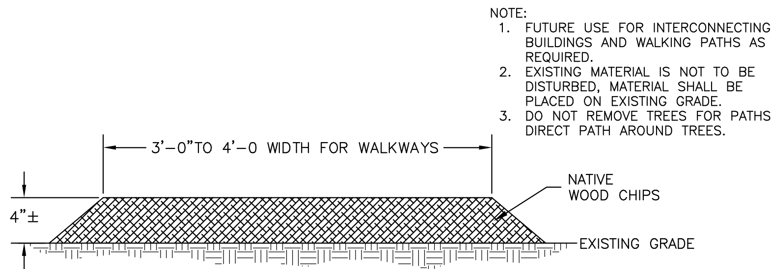
3 WOOD CHIP PATH DETAIL S-102 N.T.S.
