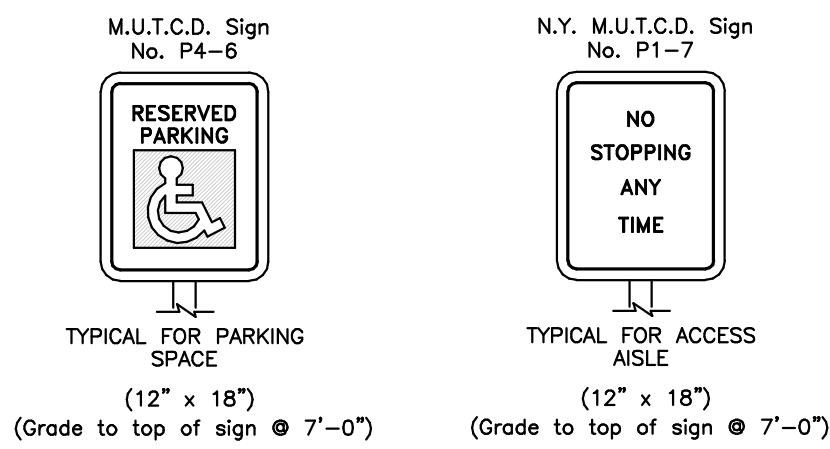
TYPICAL ADA SIGN DETAIL NOT TO SCALE
