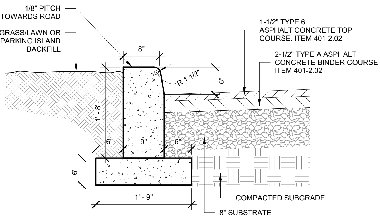
7 CURB DETAIL S-102 1" = 1'-0"
