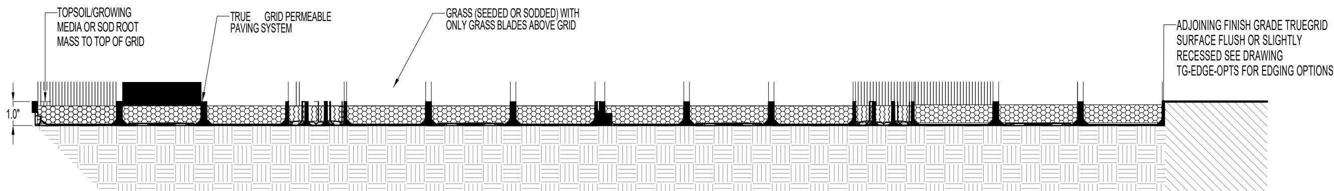
5 PARKING SPOT DEMARCATION DETAIL S-102 N.T.S.
